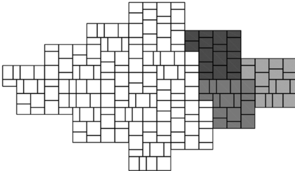
Cluster A
